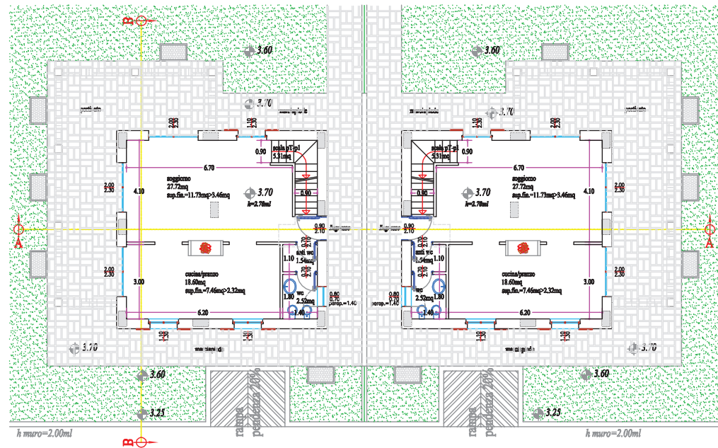
Piano terra
