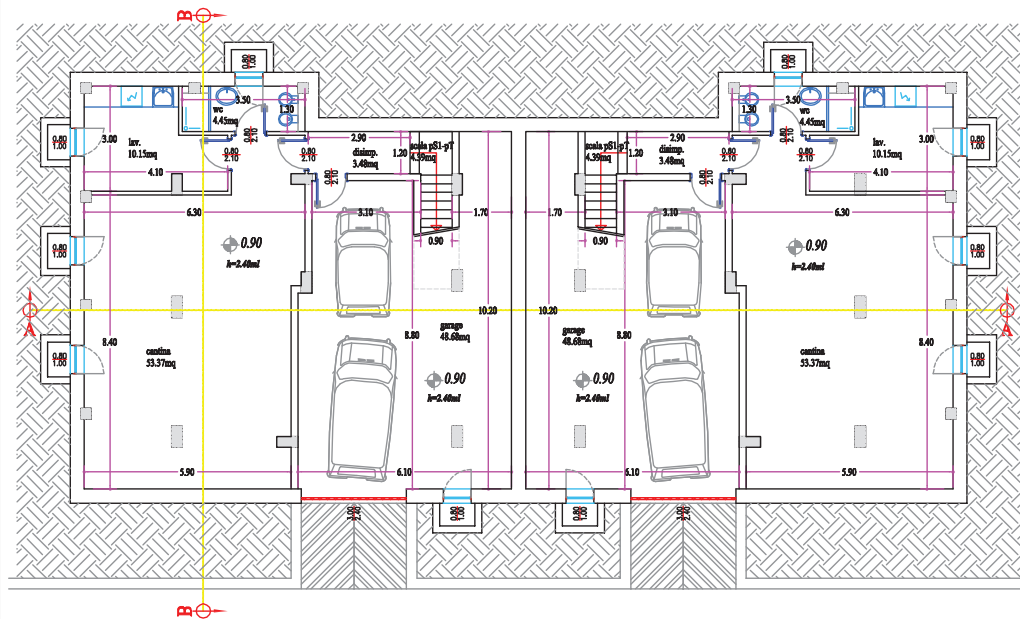
Piano interrato
