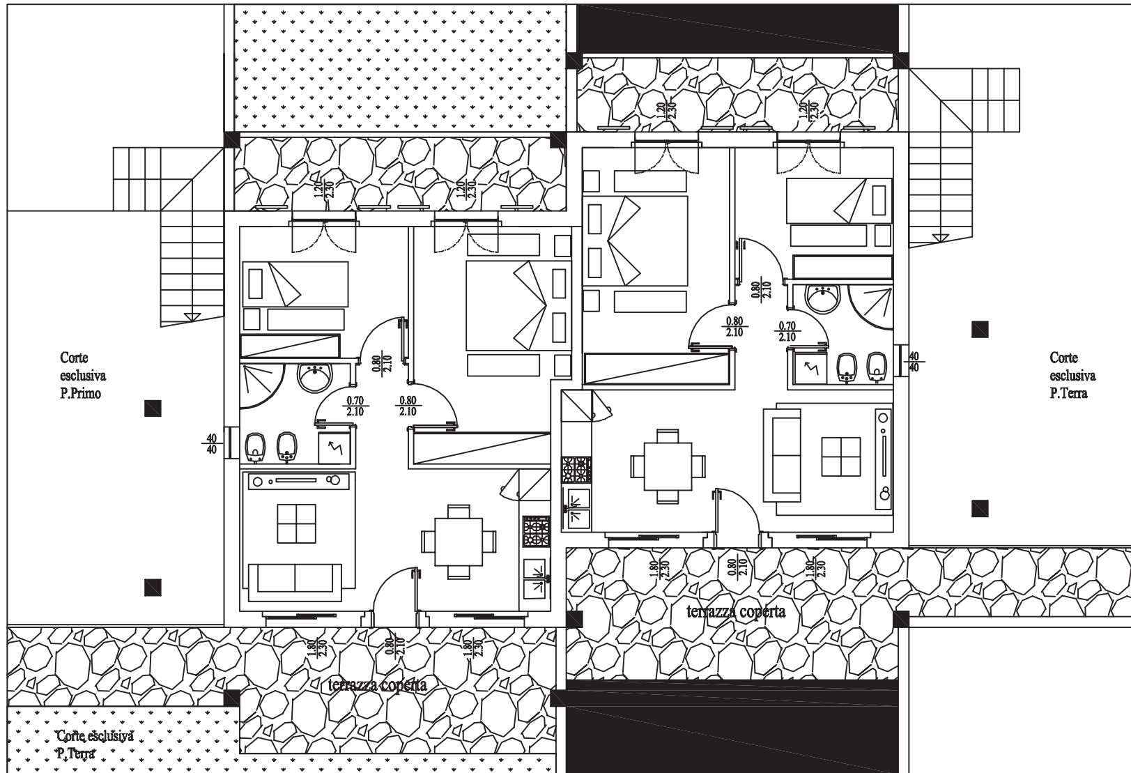
Piano terra - Lotto 2
